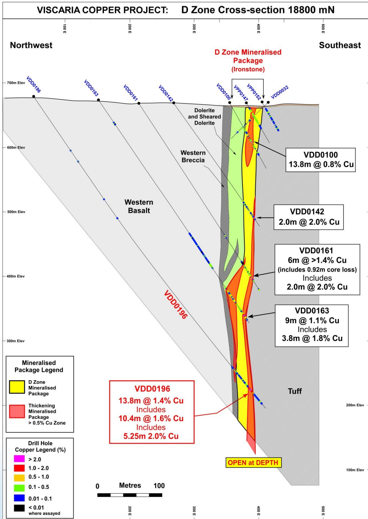
Figure 3: Drill hole cross section showing high grade intersection in hole VDD 196.
