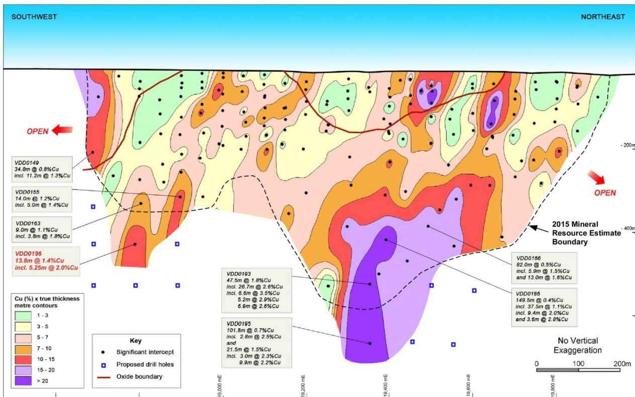
Figure 2: Location of VDD 196 on schematic long section showing Cu grade (%) x interpreted true ore zone thickness contours for D Zone ironstone hosted copper mineralisation at the Viscaria Copper Project. Quoted intercepts are downhole intervals. Southwest plunging lenses of improving grade and thickness at depth are being defined as further drilling is undertaken. The 2015 Mineral Resource estimate includes data from holes up to VDD 194 only (excludes VDD 195 and 196).
