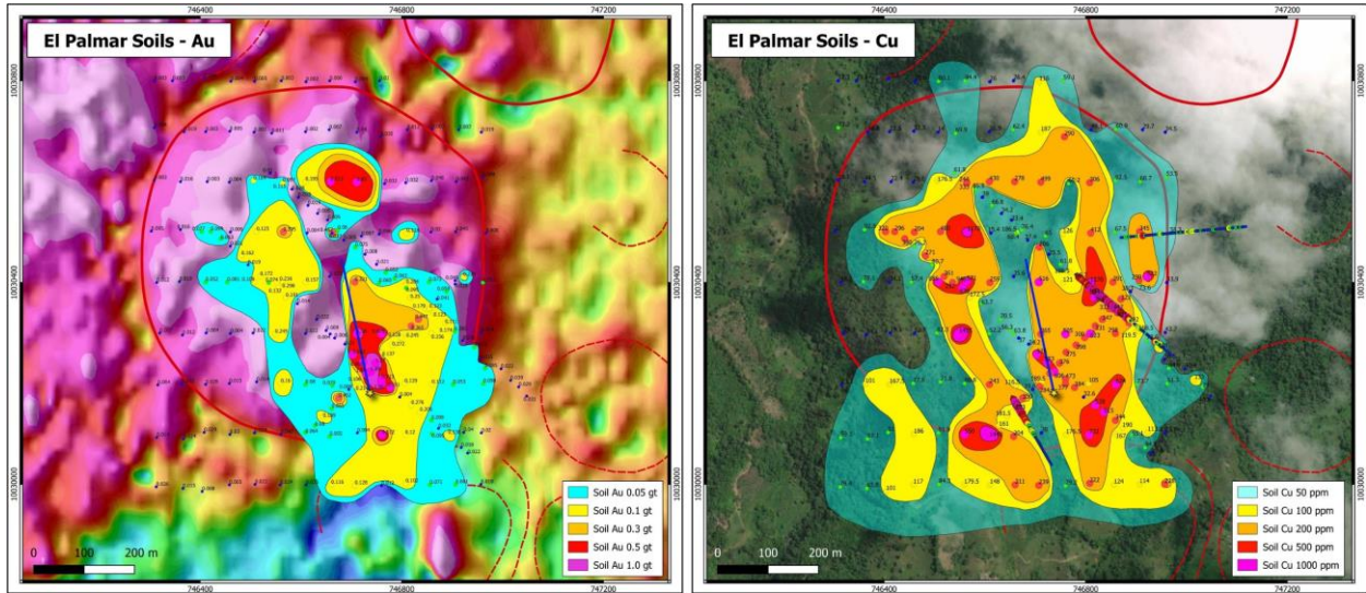
Figure 3: Side-by-side gold and copper in auger soils over the main magnetic target at El Palmar and showing the location of the first drill hole (blue trace)
