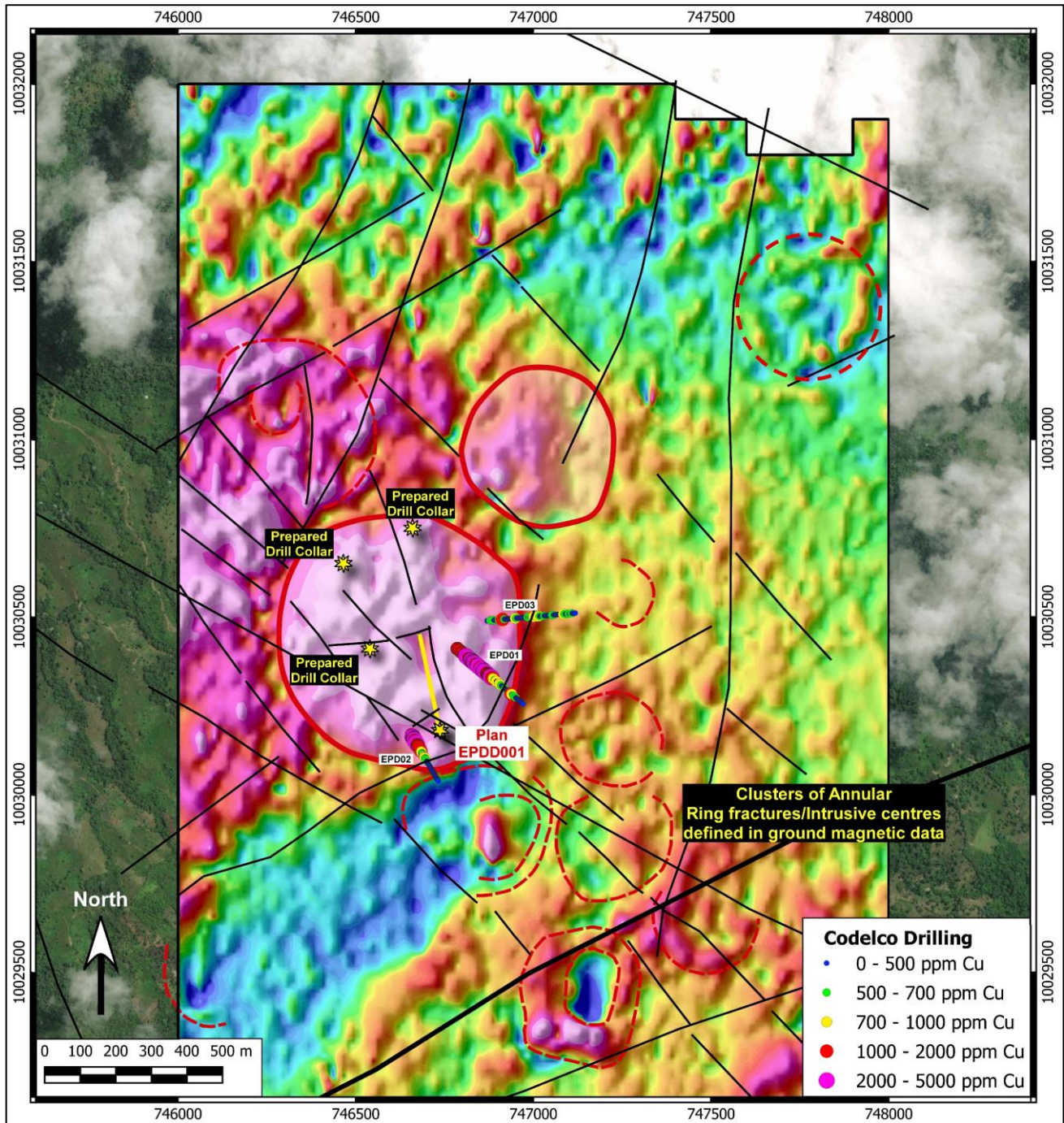
Figure 2: RTP magnetics image showing the circular magnetic anomaly being targeted with drilling. Also shown are three historical drill holes, which drilled away from the target area, and the prepared drill collars to allow for future drilling.
