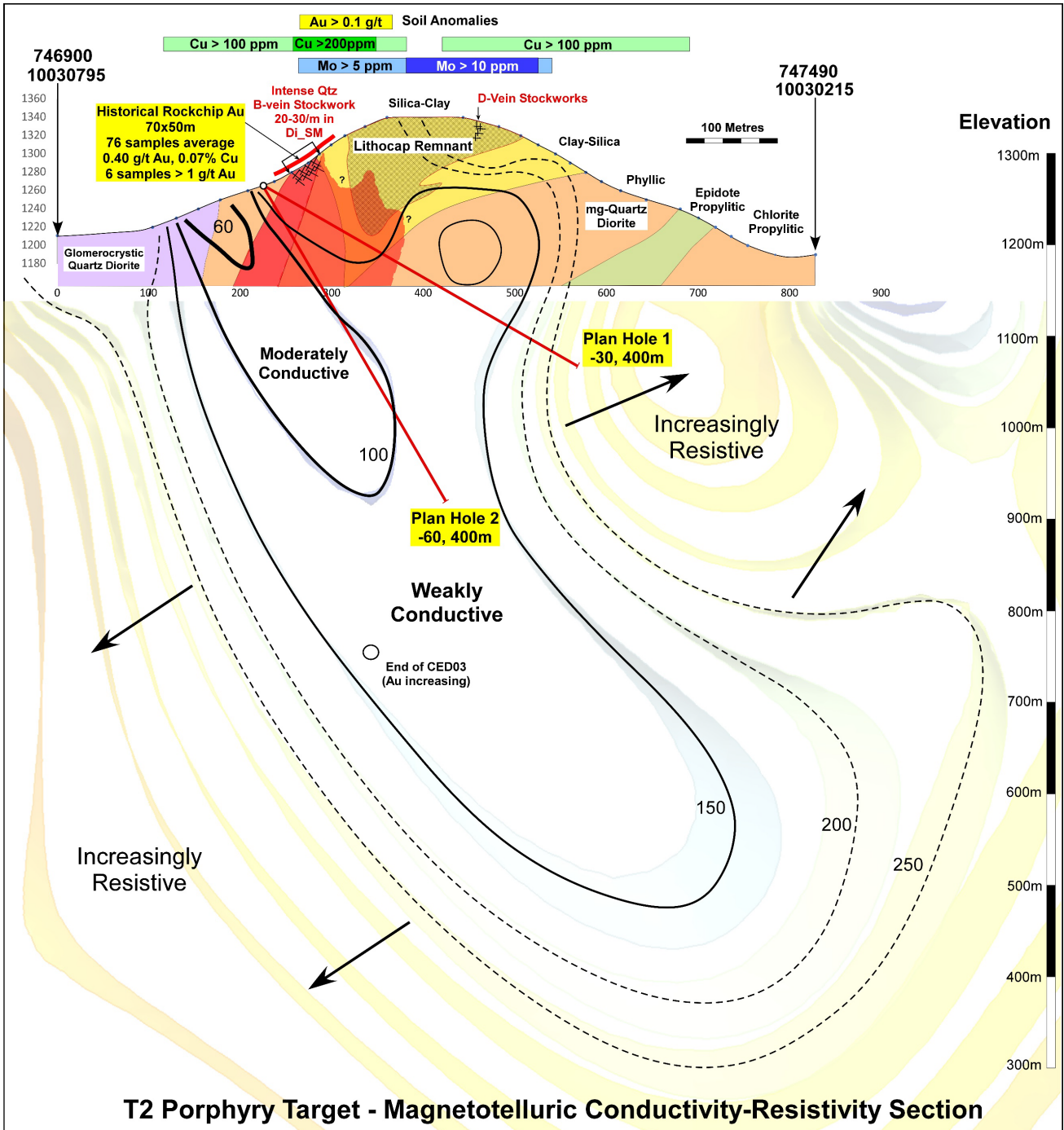
Figure 4: Cross section through the T2 target showing outcropping porphyry stockwork area with anomalous copper gold and molybdenum, coincident with a large area of weakly conductive material. Two drill holes are planned and shown on section. These will be drilled during October-November.
