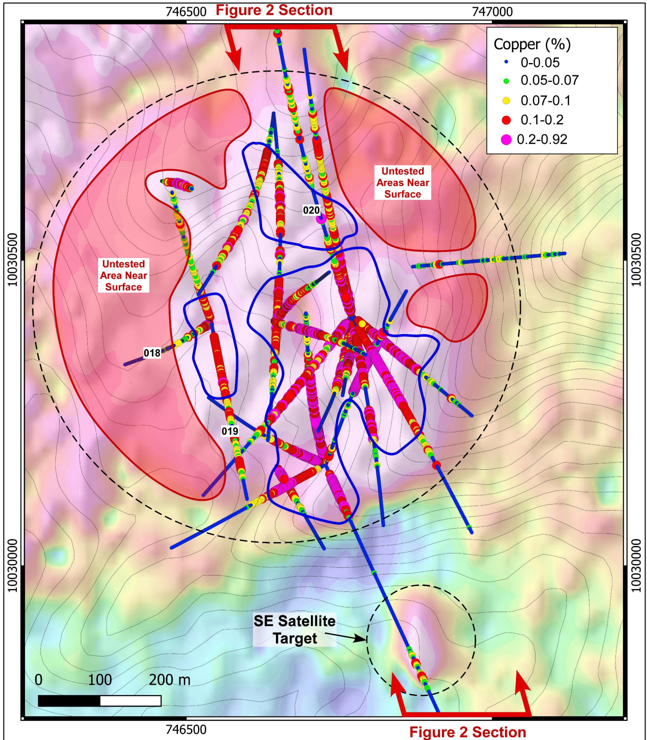
Figure 1: Drill status plan for El Palmar. Blue outline areas represent surface projection of a cluster of gold-copper mineralised porphyry domains, within a broader less well mineralised system. Areas in red outline and shading are still to be drilled.
