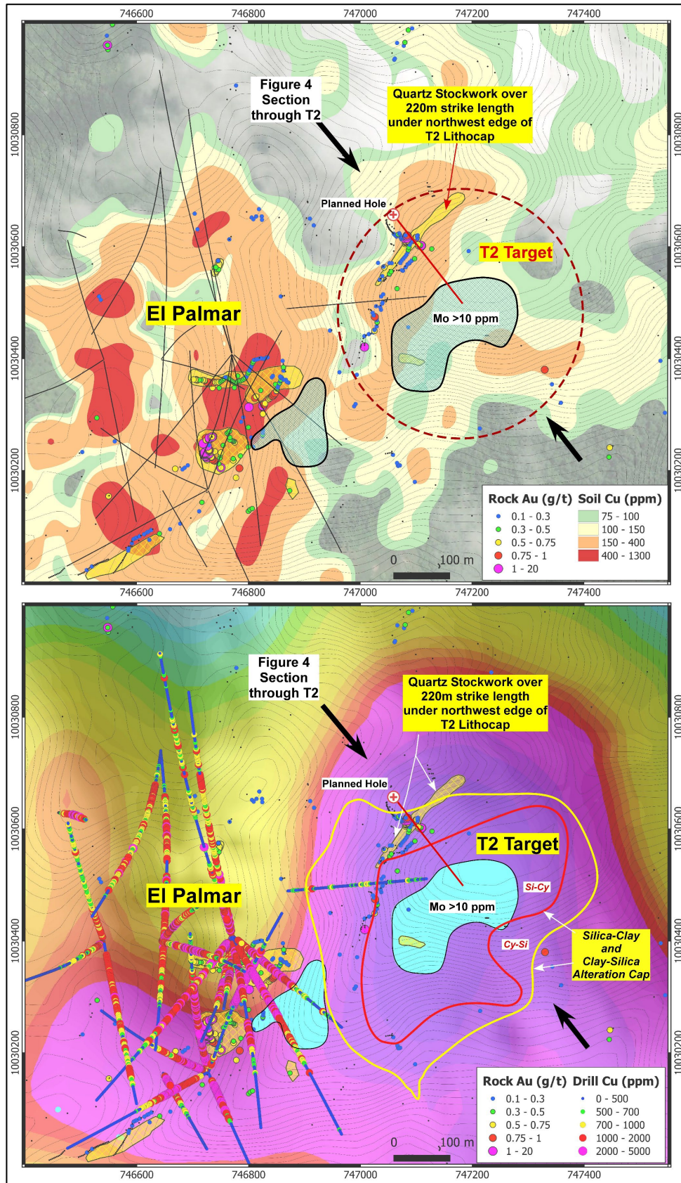
Figure 3: Plan view of the T2 target located immediately east of the area of drilling to date at El Palmar. The upper panel shows Copper-in soils with the main molybdenum anomalies, rock chip results and area of quartz stockwork mapped at T2. The lower panel background image is MT conductivity at 400m below surface.
