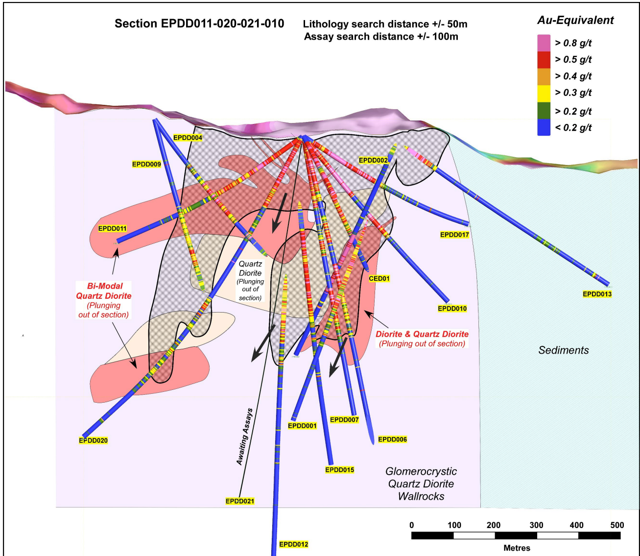
Figure 2: NNW-SSE section through holes EPDD011, 020, 021 and 010 at El Palmar. Black arrows indicate interpreted plunge of mineralisation out of the section plane. Assays for hole EPDD021 are pending.
