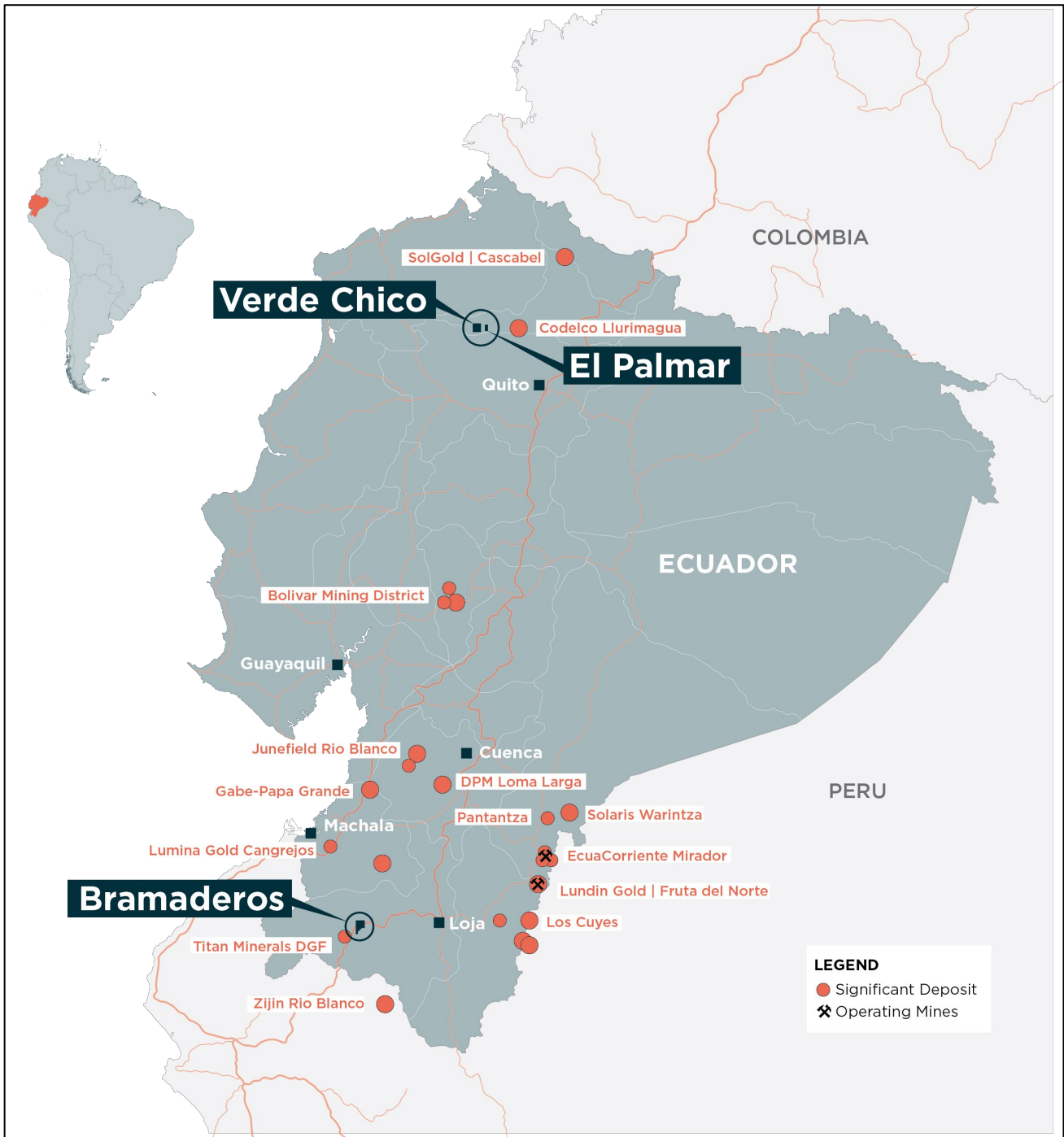
Figure 7: Location of the El Palmar project in northern Ecuador, the Verde Chico project nearby, and the Bramaderos Project in southern Ecuador.
