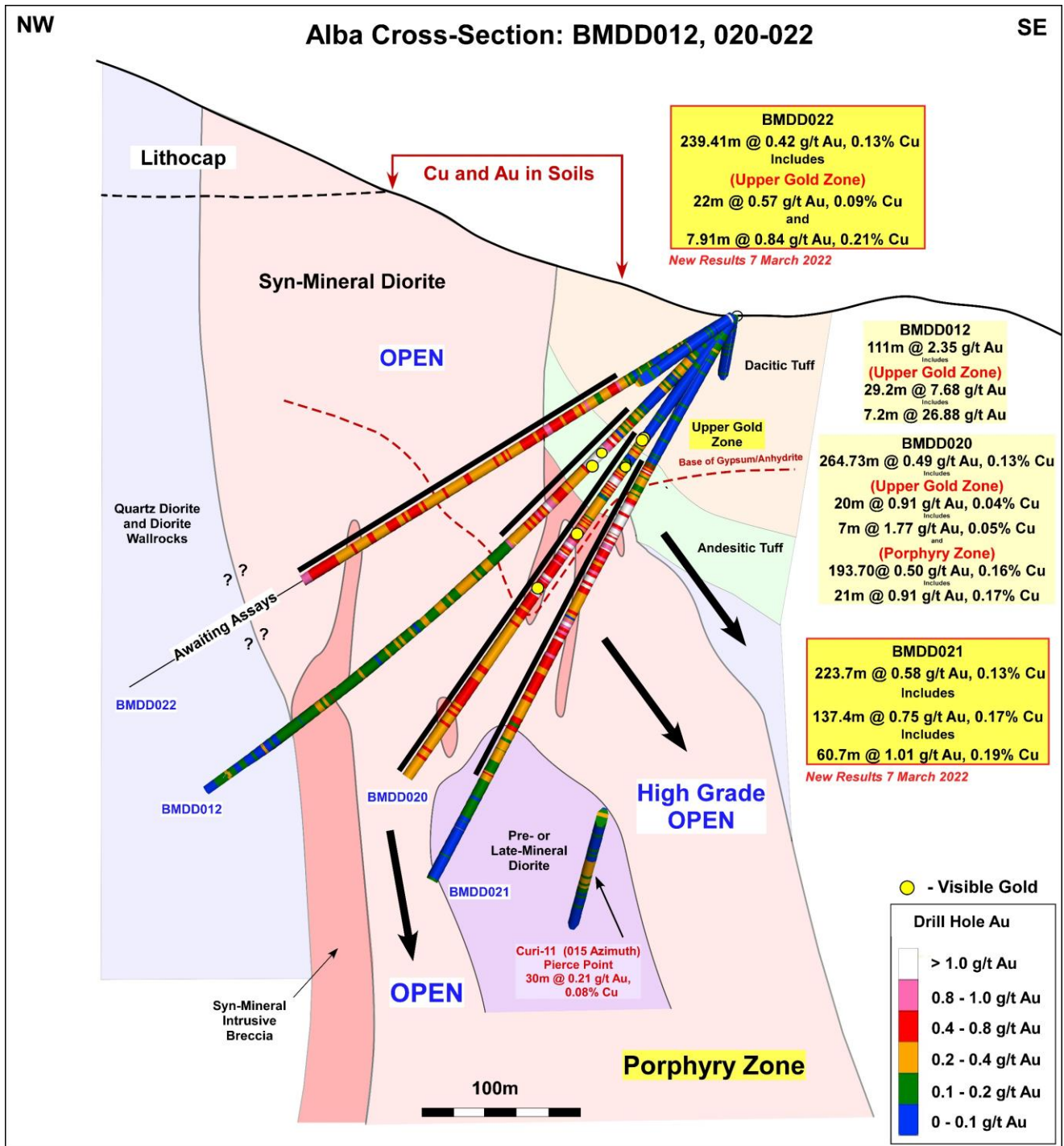
Figure 2: Alba cross section showing drill holes BMDD012, 20, 21, and 22. Hole BMDD022 finished in high-grade mineralisation and has subsequently been deepened with assays pending for the extension interval.
