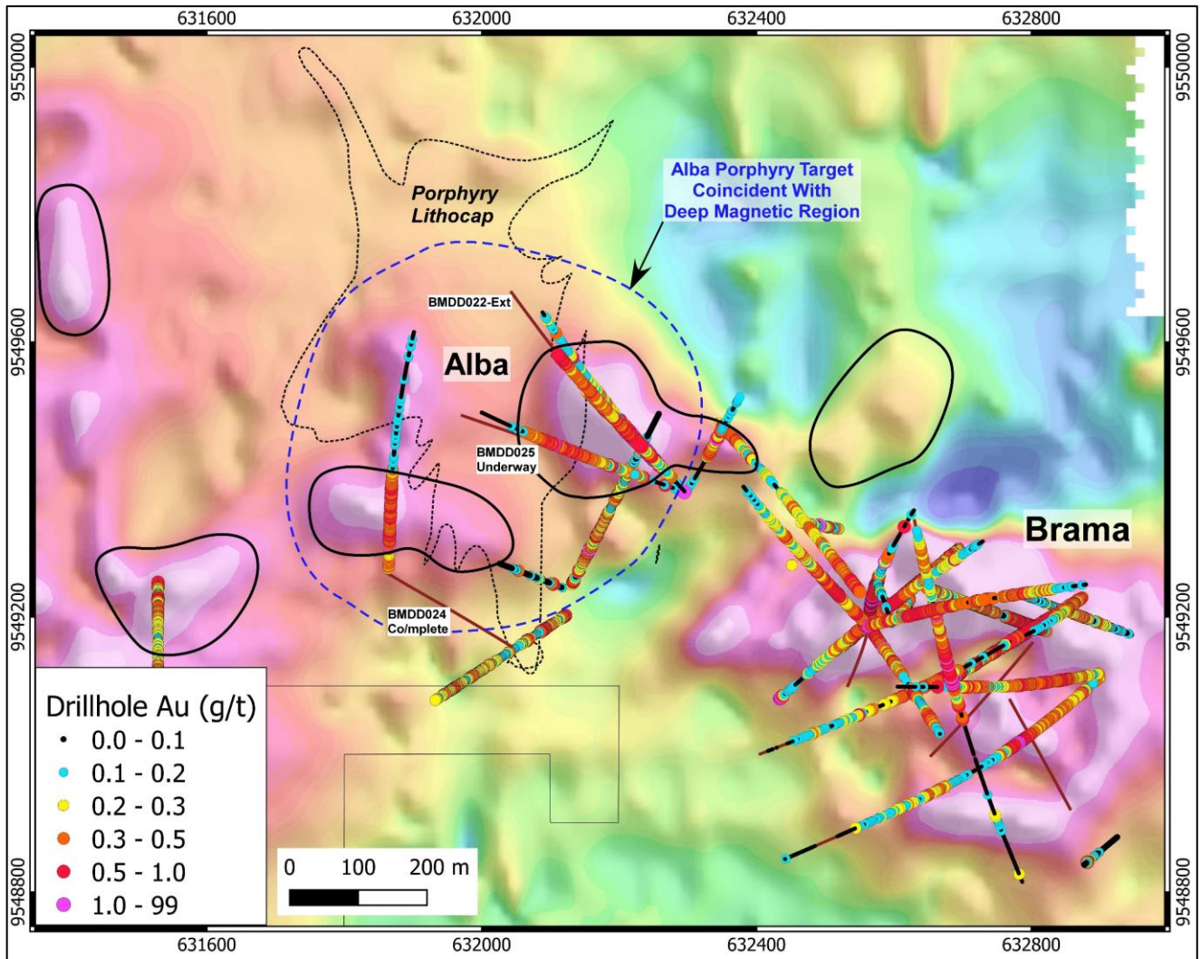
Figure 1: Alba target drill status plan showing the interpreted porphyry gold-copper target zones, located adjacent to the Brama porphyry gold-copper system.
