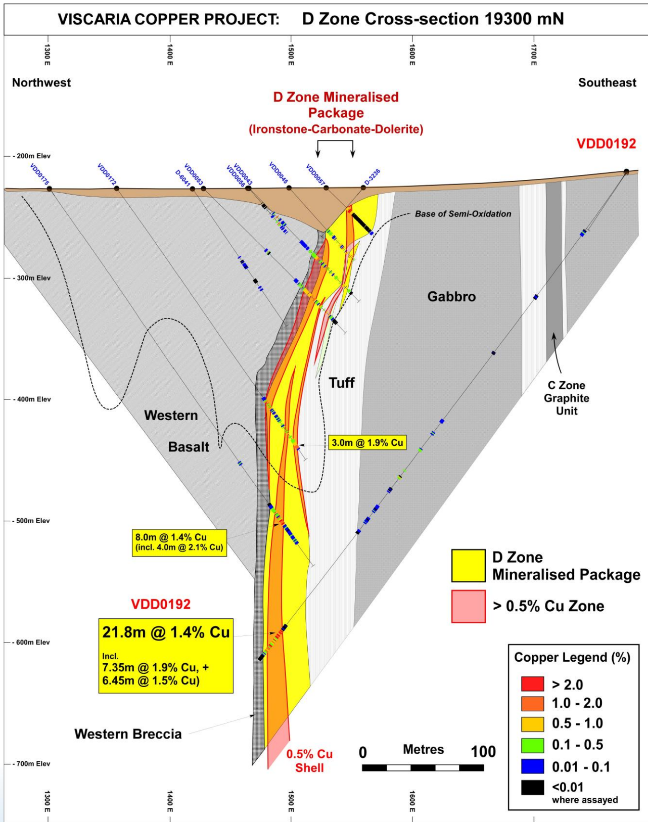
Figure 3: Drill hole cross section containing hole VDD 192.
